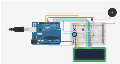
Schema Tinkercad
