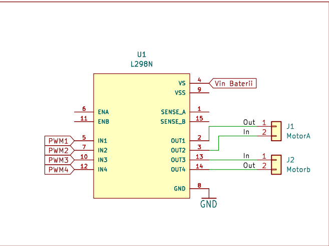
File: L298N_project.kicad_sch
