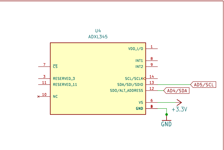
File: adxl345_project.kicad_sch
