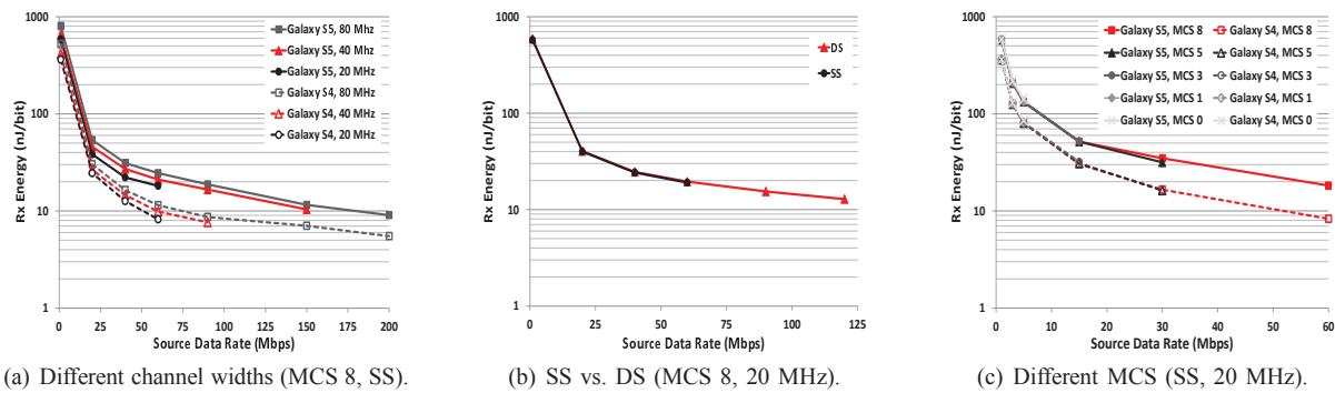
Fig. 7. Energy per bit comparison as a function of the source data rate for Galaxy S4 and Galaxy S5.
