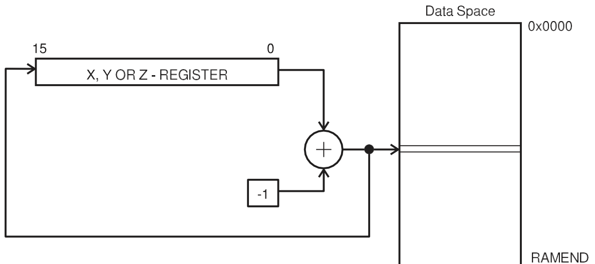
Figure 2-7. Data Indirect Addressing with Pre-decrement
