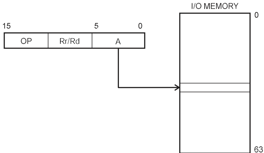
Figure 2-3. I/O Direct Addressing
