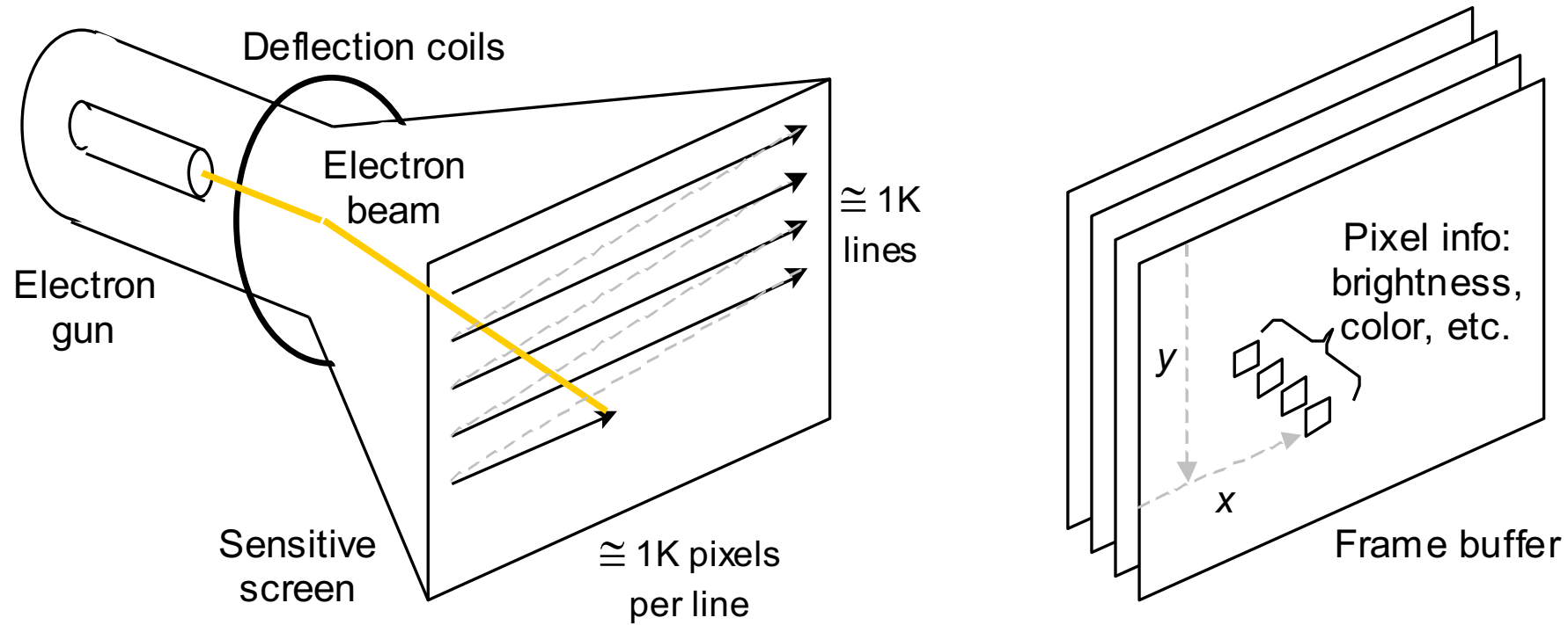
(a) Image formation on a CRT
