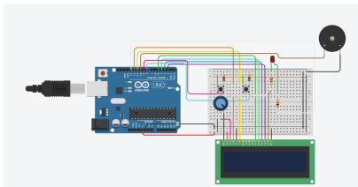
Schema Tinkercad
