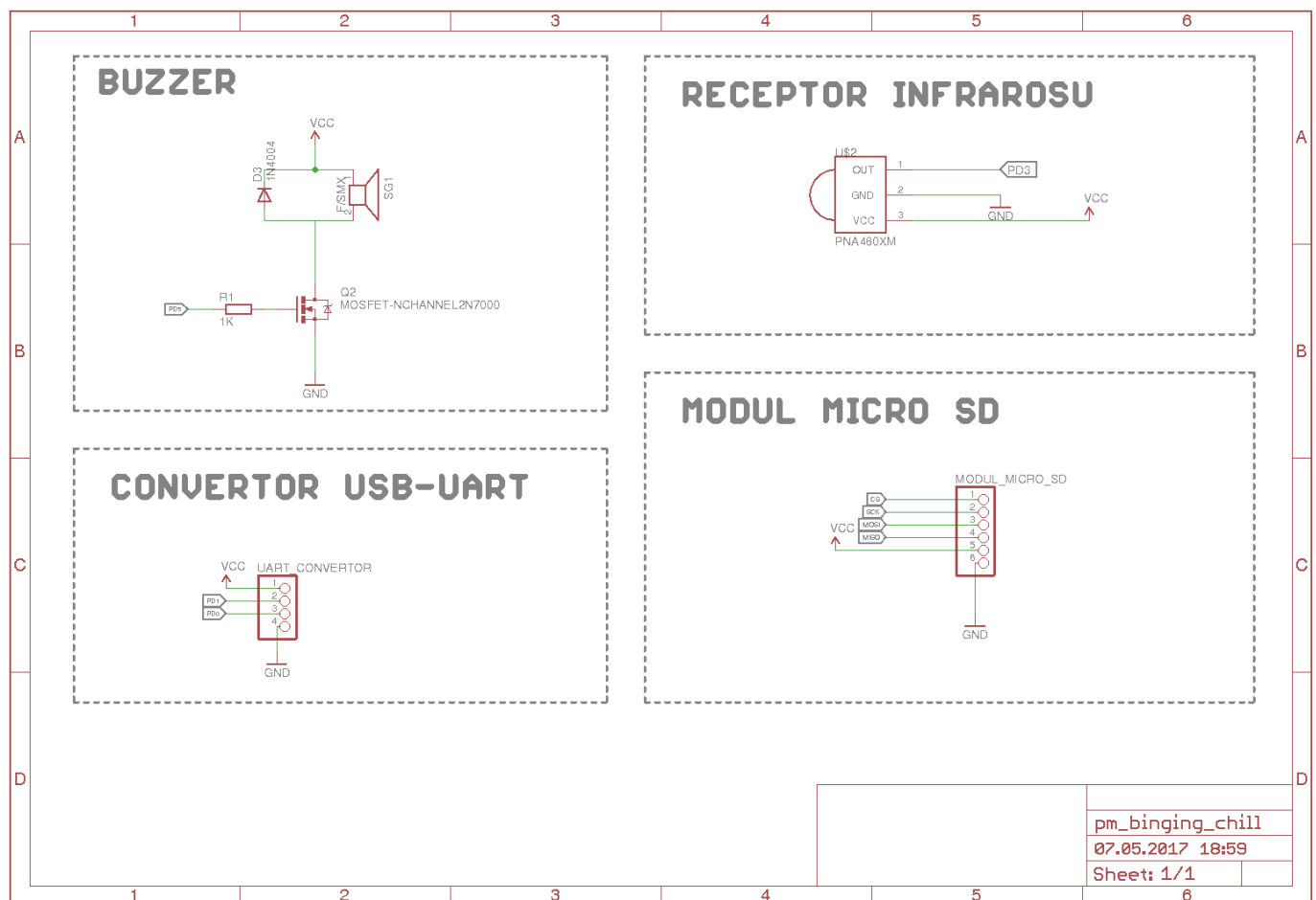
Schema electrica
